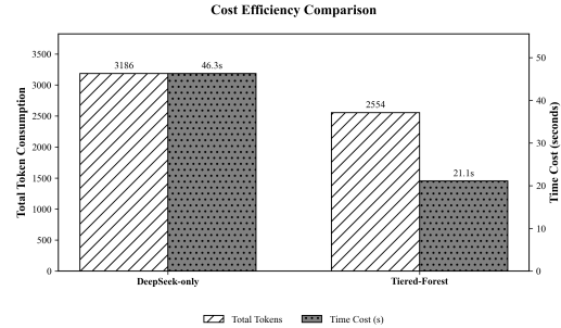
Figure 4: Comparison of computational cost (tokens) and latency, highlighting the efficiency of the tiered approach.
